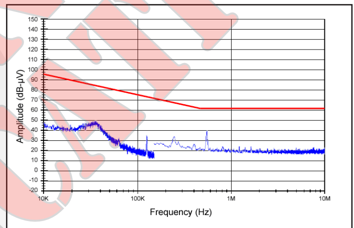
Figure 4: MIL-STD-461E Method CE102 High Frequency Conducted Emissions. Limit line (in red) is the 'Basic Curve'.
