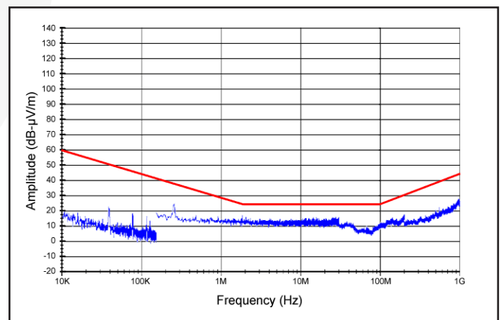
Figure 6: MIL-STD-461E Method RE102 High Frequency Radiated Emissions. Limit line (in red) is the 'Submarine External to Pressure Hull Curve'.
