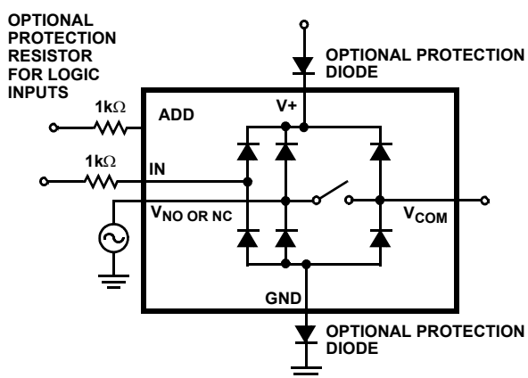
FIGURE 8. OVERVOLTAGE PROTECTION
