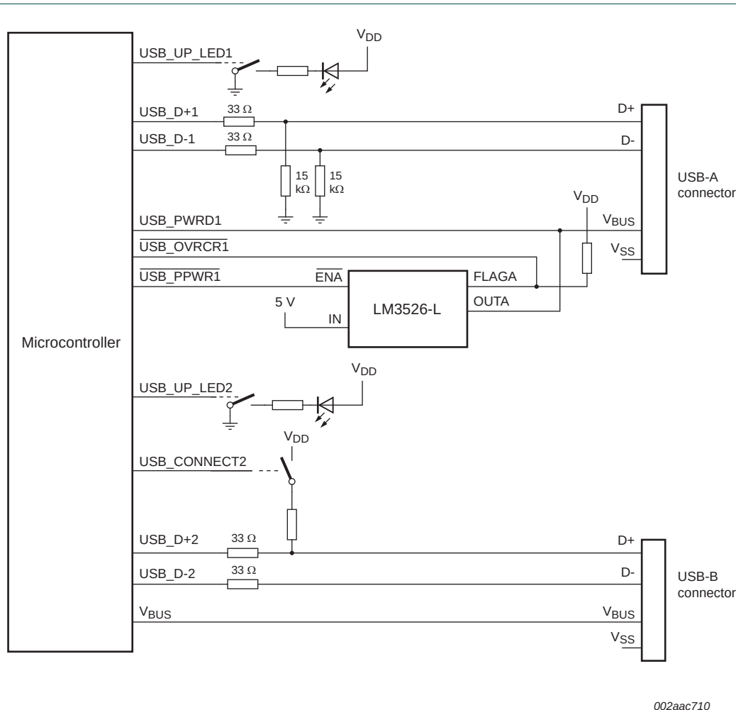
Fig 52. USB device port configuration: port U1 host and port U2 device
