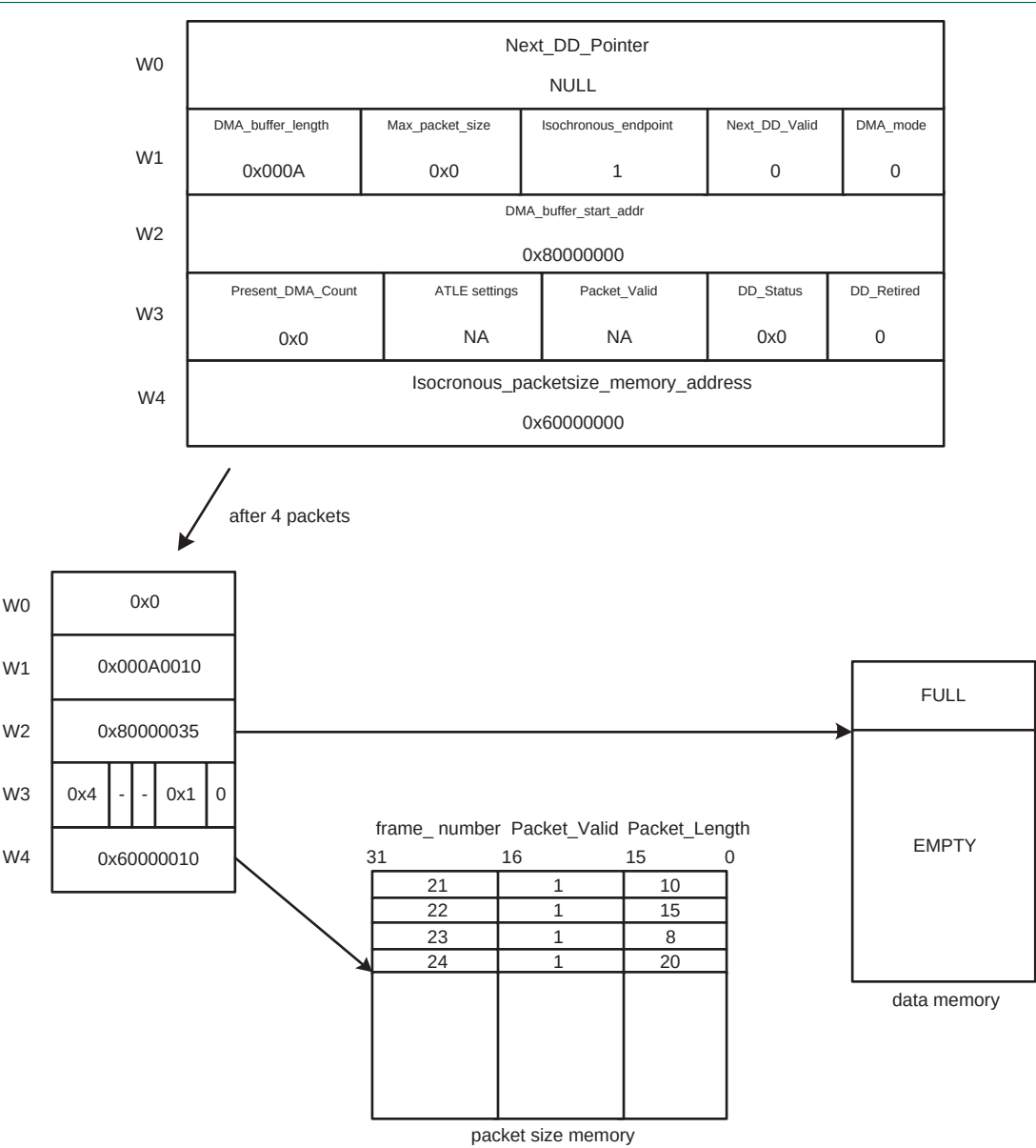
Fig 45. Isochronous OUT endpoint operation example
