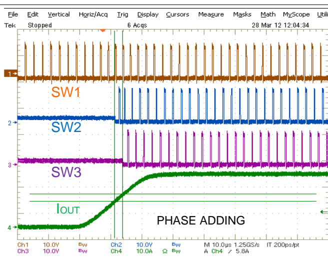
Figure 120. Phase Adding
