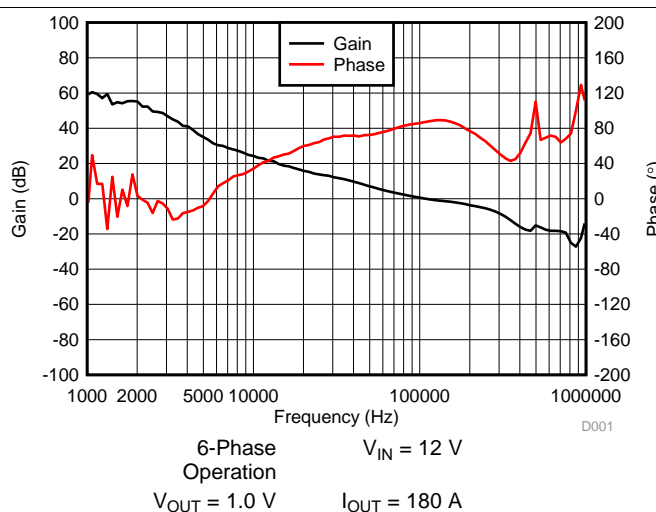
Figure 122. Bode Plot
