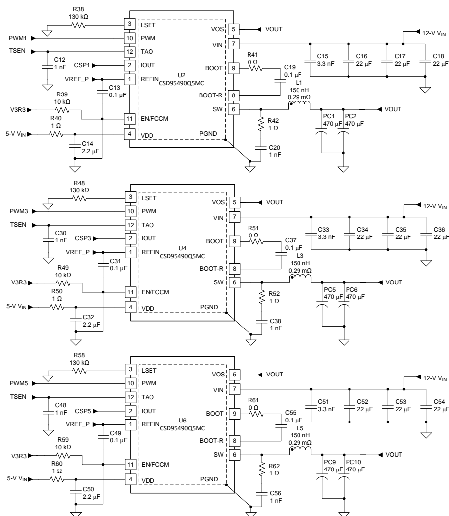
Figure 104. Power Stage Schematic for a 6-Phase, 1 V, 180 A Application
