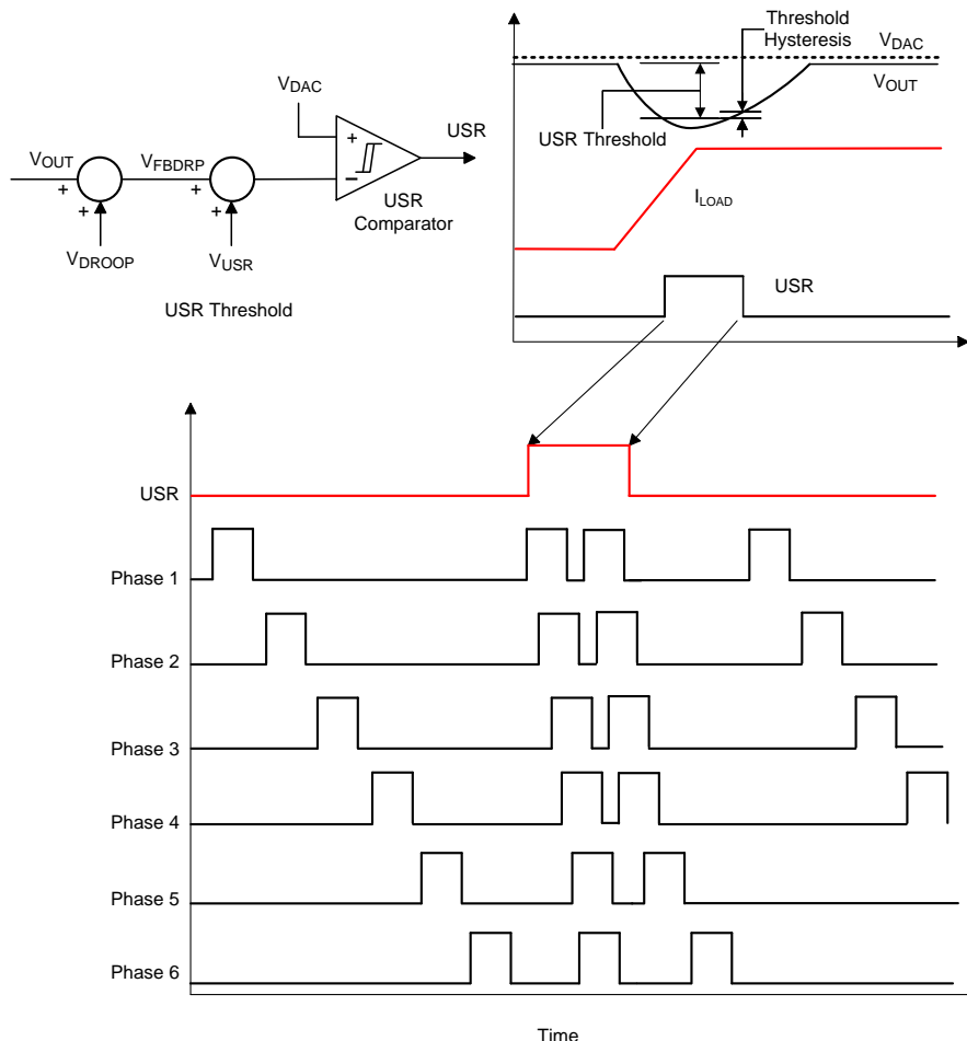
图 14. Performance for a Load Transient Step-up With USR Enabled
