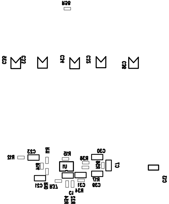
Figure 46. PCB Bottom-Side Silkscreen
