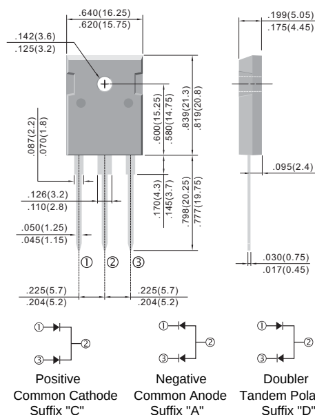
TO-3P/TO-247AD
