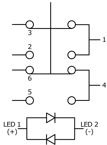
SCHEMATIC ▲ ON - ON DPDT Illuminated RED (FORWARD) / GREEN (REVERSE)
