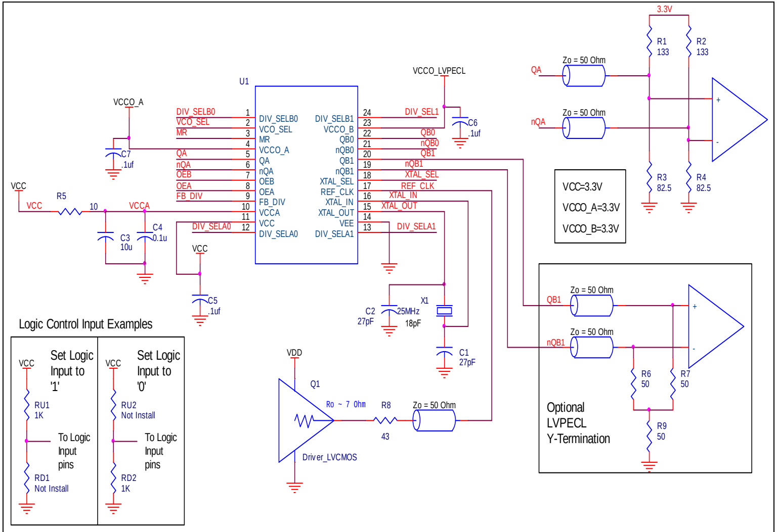
Figure 6. 8433625 Schematic Example
