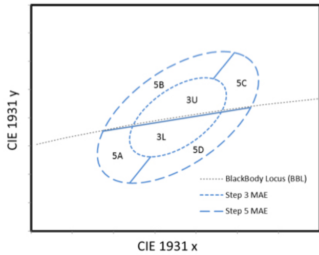
Figure 6: Color bin definition for LUXEON FlipChip White at 80 CRI.
