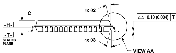
VIEW AA
