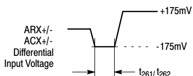
Figure 39. ARX/ACX Timing
