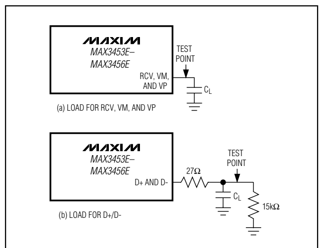
Figure 6. Test Circuits
