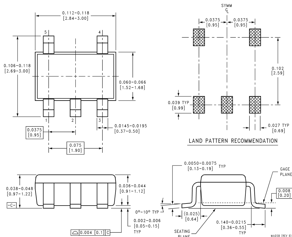
5-Pin SOT23-5 NS Package Number MA05B
