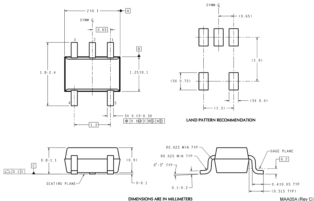
5-Pin SC70-5 NS Package Number MAA05A
