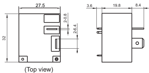
Outline Dimensions
