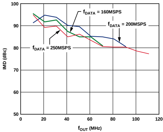
Figure 18. AD9779A Third-Order IMD vs. f_{OUT} , 1× Interpolation
