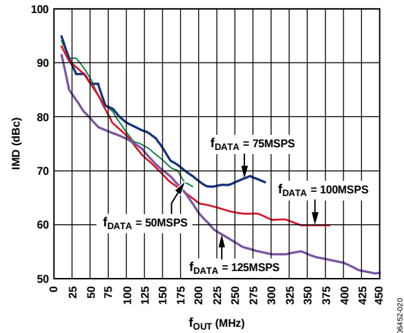
Figure 21. AD9779A Third-Order IMD vs. f_{OUT} , 8× Interpolation
