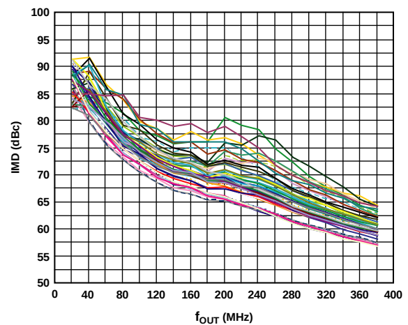
Figure 23. AD9779A Third-Order IMD vs. f_{OUT} , Over 50 Parts, 4× Interpolation, f_{DATA} = 200 MSPS
