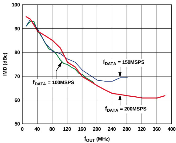
Figure 20. AD9779A Third-Order IMD vs. f_{OUT} , 4× Interpolation
