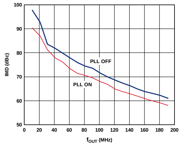
Figure 22. AD9779A Third-Order IMD vs. f_{OUT} , 4× Interpolation, f_{DATA} = 100 MSPS, PLL On/Off
