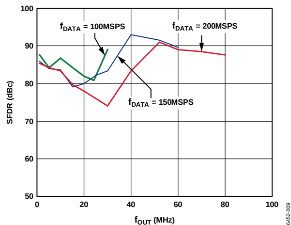
Figure 10. AD9779A In-Band SFDR vs. f_{OUT} , 4x Interpolation
