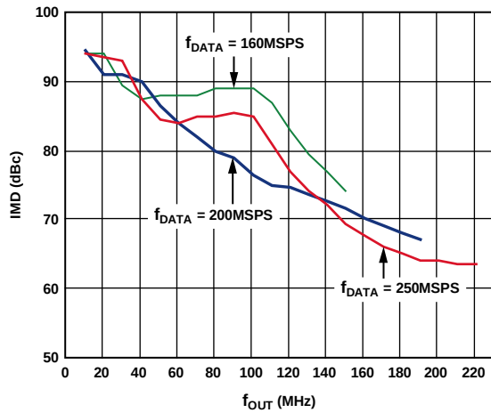
Figure 19. AD9779A Third-Order IMD vs. f_{OUT} , 2× Interpolation
