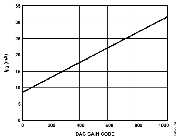
Figure 77. I_{\text{FS}} vs. DAC Gain Code
