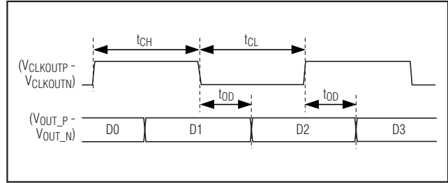
Figure 5. Serialized Output Detailed Timing Diagram
