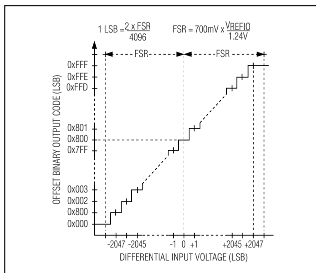
Figure 7. Bipolar Transfer Function with Offset Binary Output Code ( \bar{T}/B = 1 )
