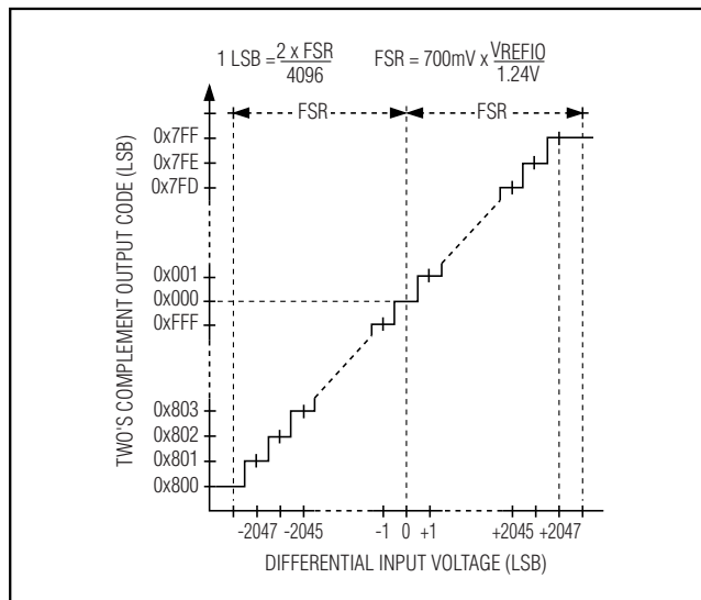
Figure 6. Bipolar Transfer Function with Two's Complement Output Code ( \bar{T}/B = 0 )
