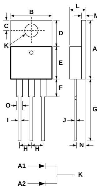
TO-220AB
