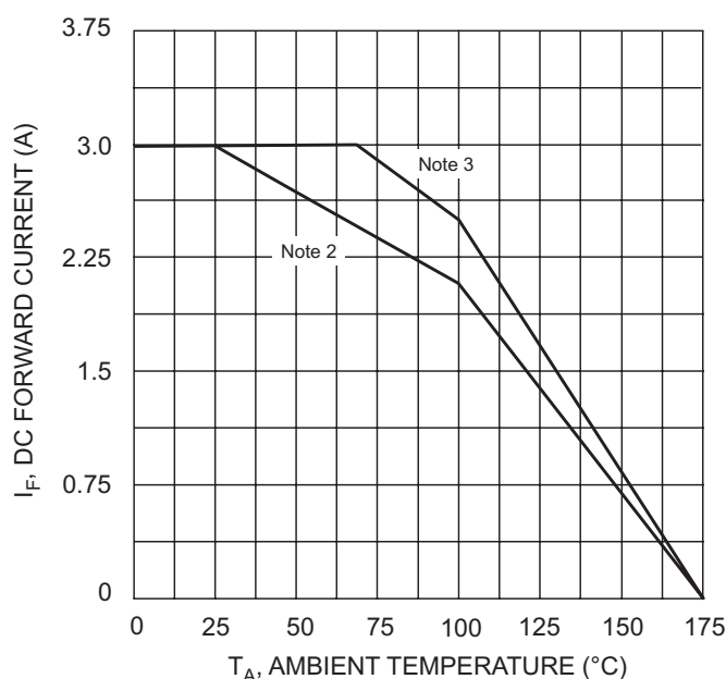
T_A , AMBIENT TEMPERATURE ( ^\circ\text{C} ) Fig. 4 DC Forward Current Derating, per element
