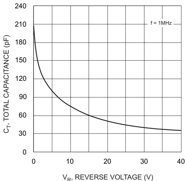
V_R , REVERSE VOLTAGE (V) Fig. 3 Typical Total Capacitance vs. Reverse Voltage, per element
