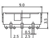
SB1SR SMT Horizontal Slide Switch
