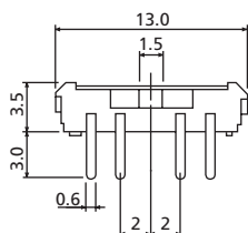
SB2HR THT, Horizontal Slide Switch
