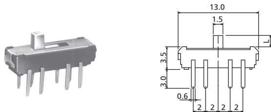
SB2HT THT, Vertical Slide Switch
