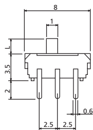
SB1HT THT Vertical Slide Switch
