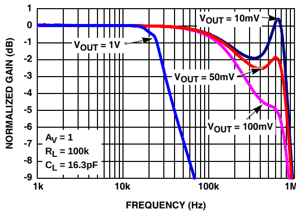
FIGURE 7. GAIN vs FREQUENCY vs V_{OUT}
