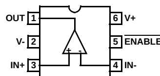
ISL28166 (6 LD SOT-23) TOP VIEW
