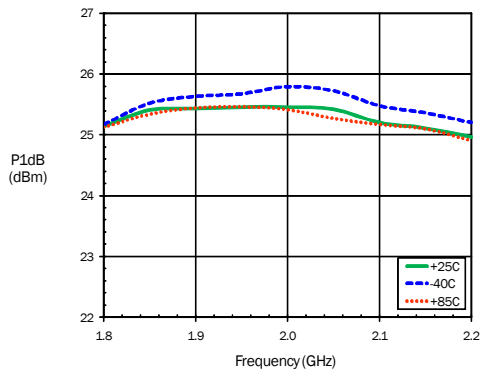
P1dB over Temperature, Max Gain
