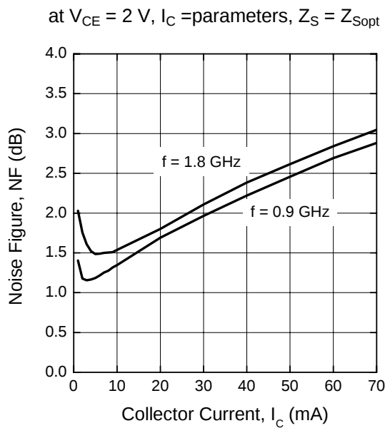
Noise Figure vs. Collector Current
