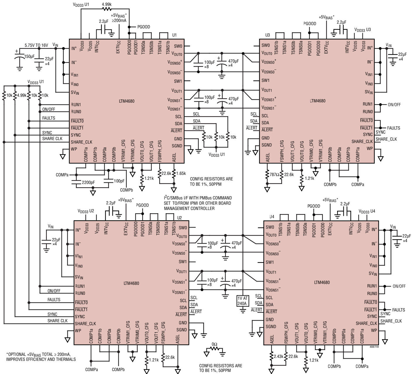
Figure 49. 8-Phase Operation with Four LTM4680 Producing 1V at 240A. Power System Management Features Accessible Through LTM4680 Over 2-Wire I²C/SMBus/PMbus Serial Interface
