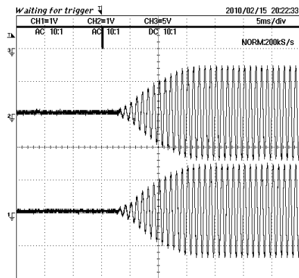
Figure 15. Advanced Switch 1
