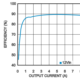
Efficiency V_{IN} = 12V , V_{OUT} = 3.3V
