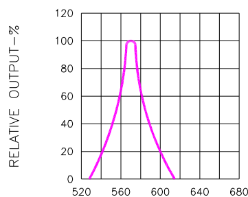
Fig.2 SPECTRAL RESPONSE
