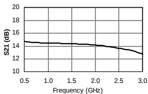
FIGURE 3. |S21| vs FREQUENCY
