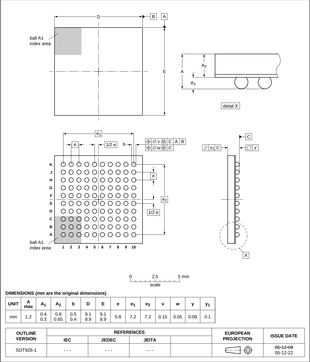
Fig 45. Package outline of the TFBGA100 package
