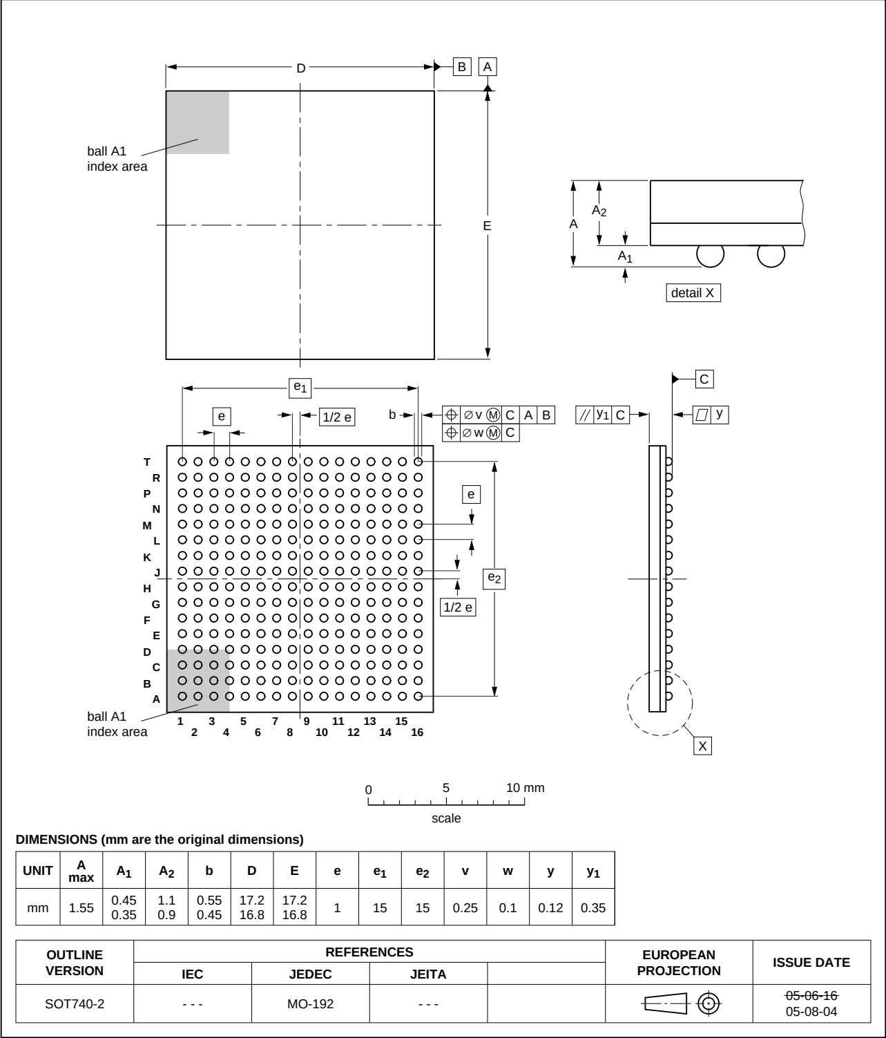
Fig 42. Package outline LBGA256 package
