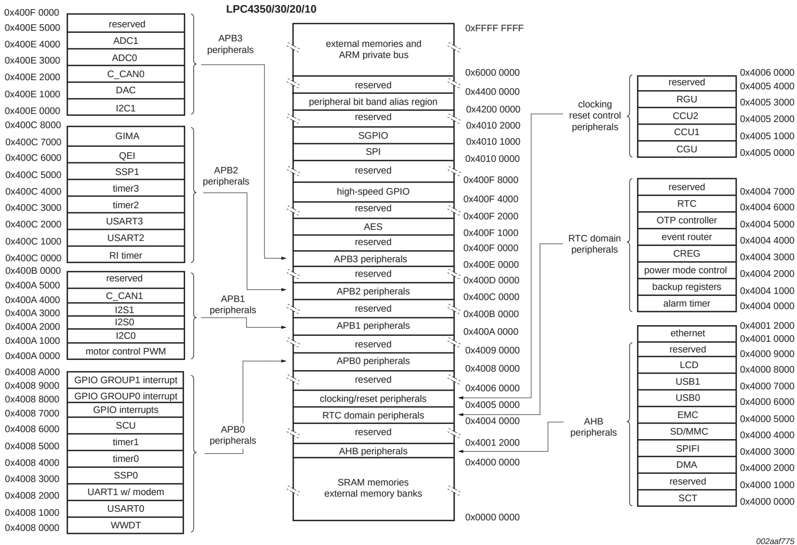
Fig 10. LPC4350/30/20/10 Memory mapping (peripherals)
