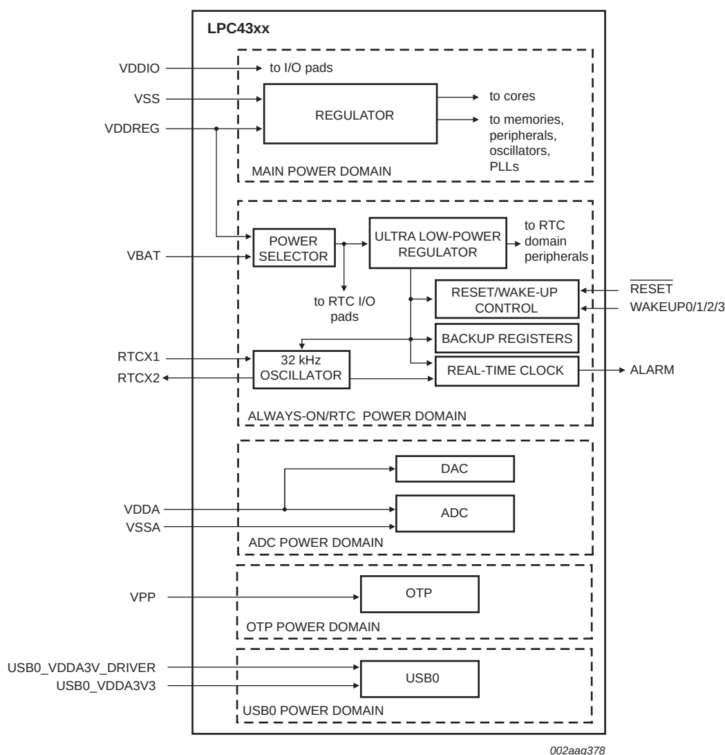
Fig 11. Power domains
