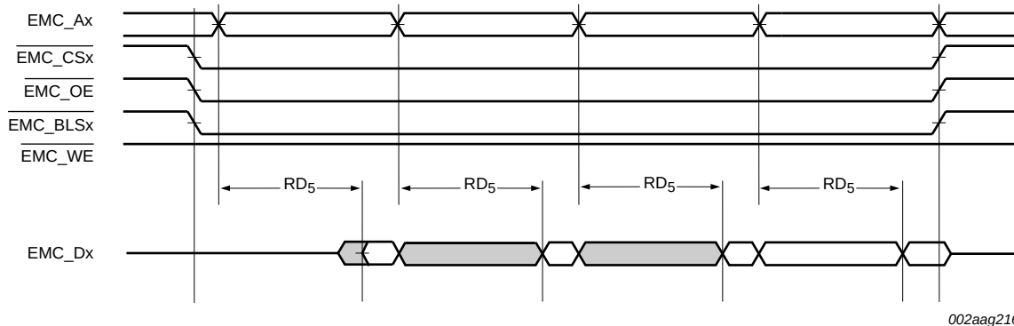
Fig 35. External static memory burst read cycle
