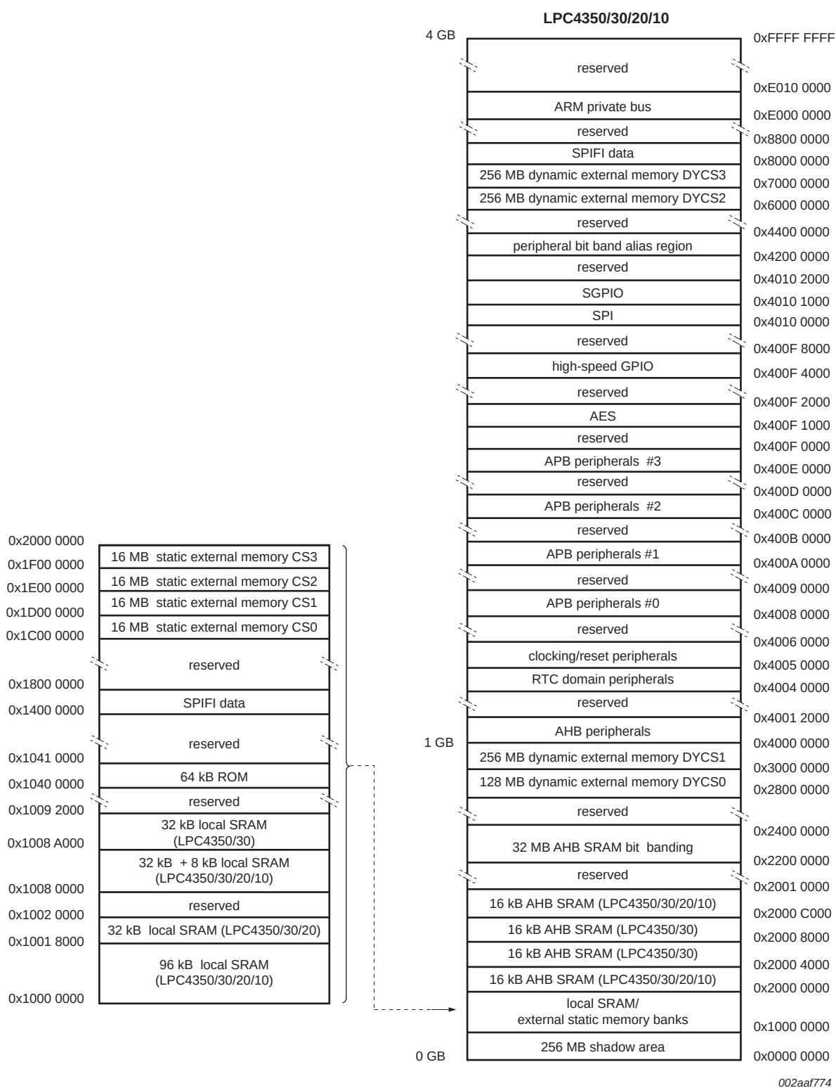
Fig 9. LPC4350/30/20/10 Memory mapping (overview)
