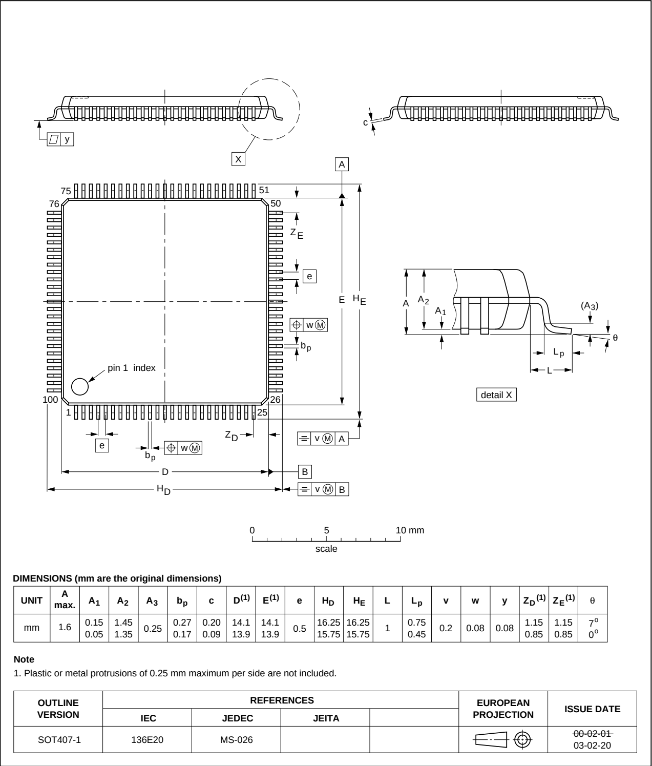
Fig 47. Package outline for the LQFP100 package
