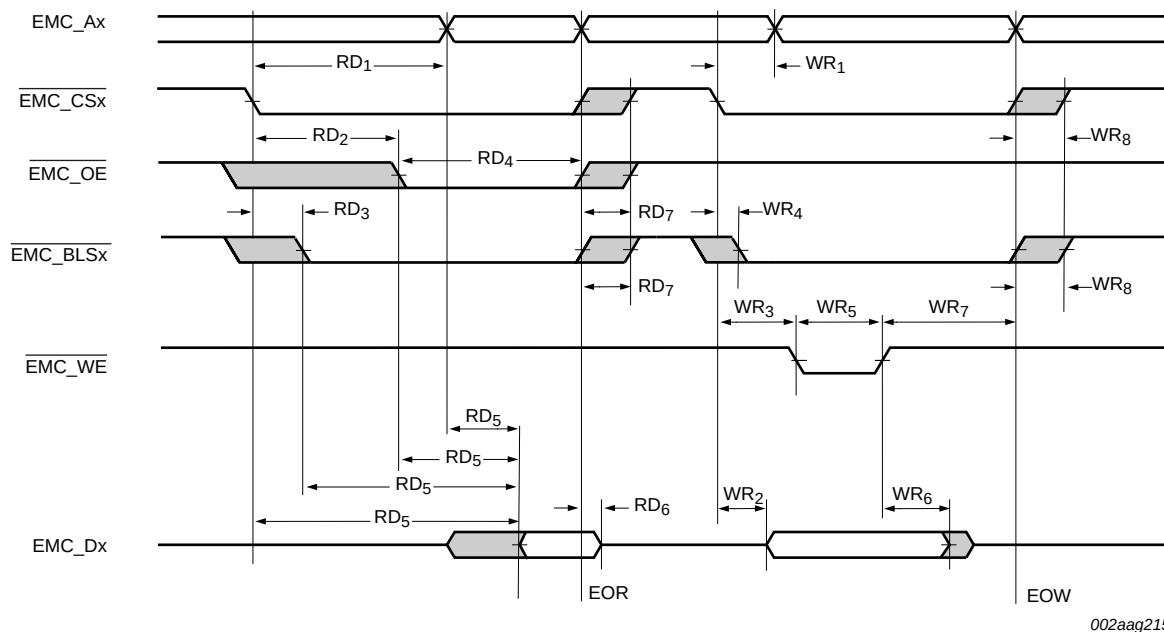
Fig 34. External static memory read/write access (PB = 1)
