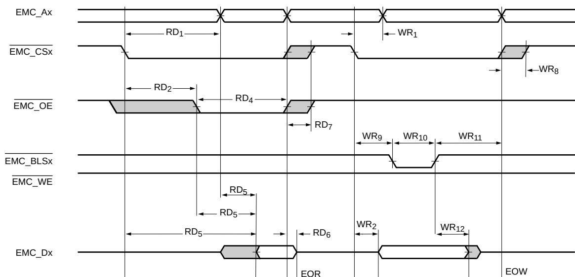
Fig 33. External static memory read/write access ( \text{PB} = 0 )
