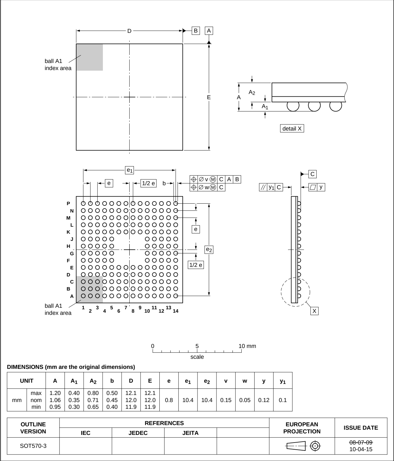
Fig 43. Package outline of the TFBGA180 package
