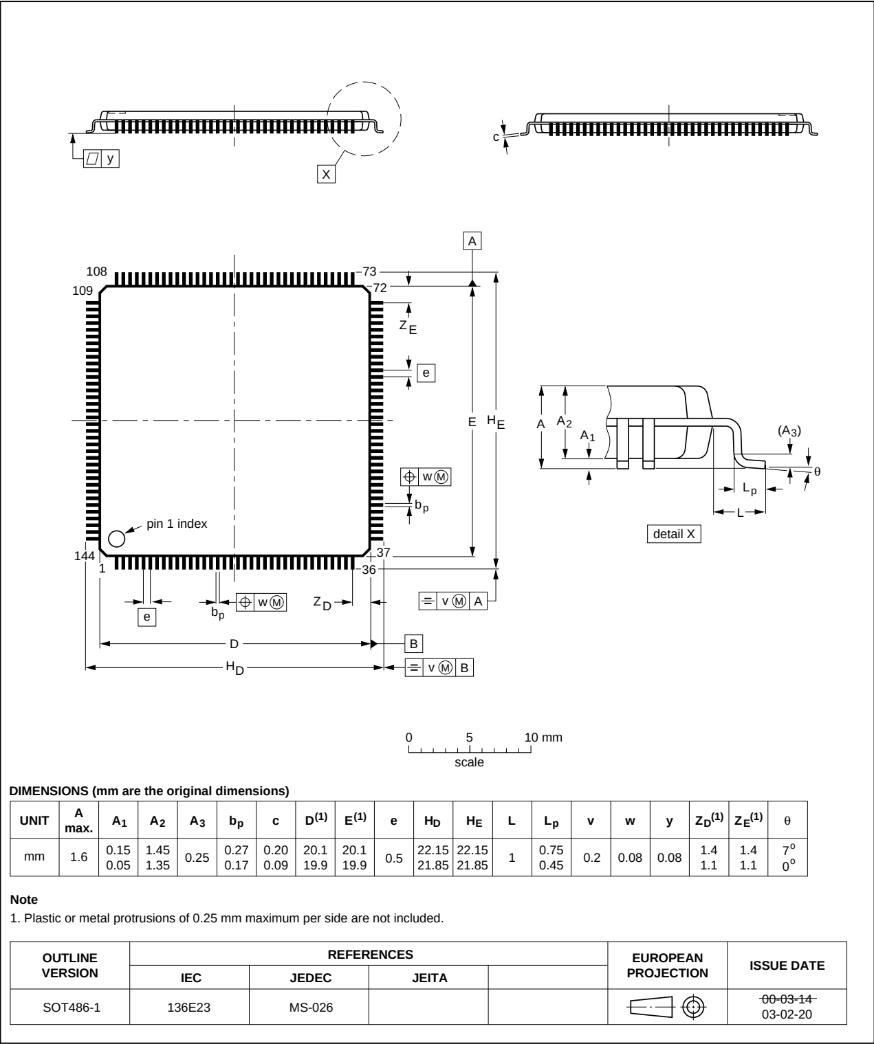
Fig 46. Package outline for the LQFP144 package
