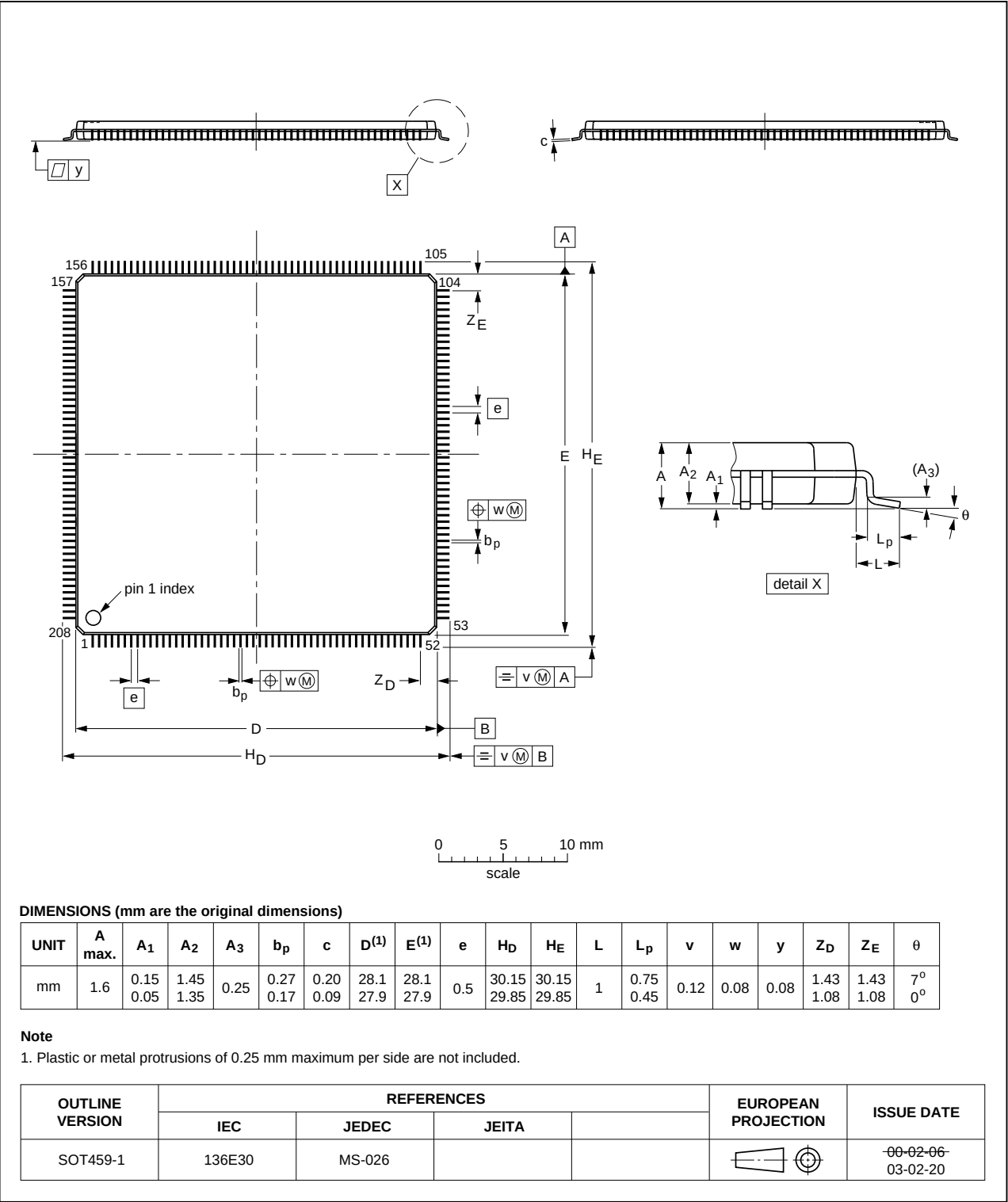
Fig 44. Package outline of the LQFP208 package
