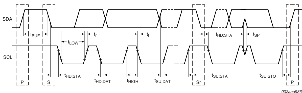
Fig 16. Definition of timing on the I 2 C-bus
