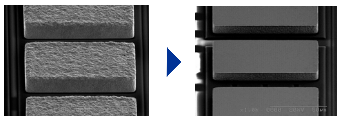
Before planarization
