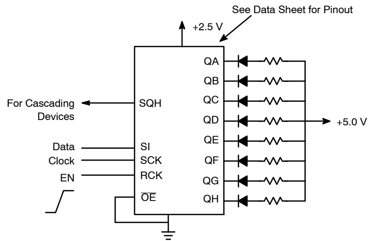
Figure 16. NLSF595 Example
