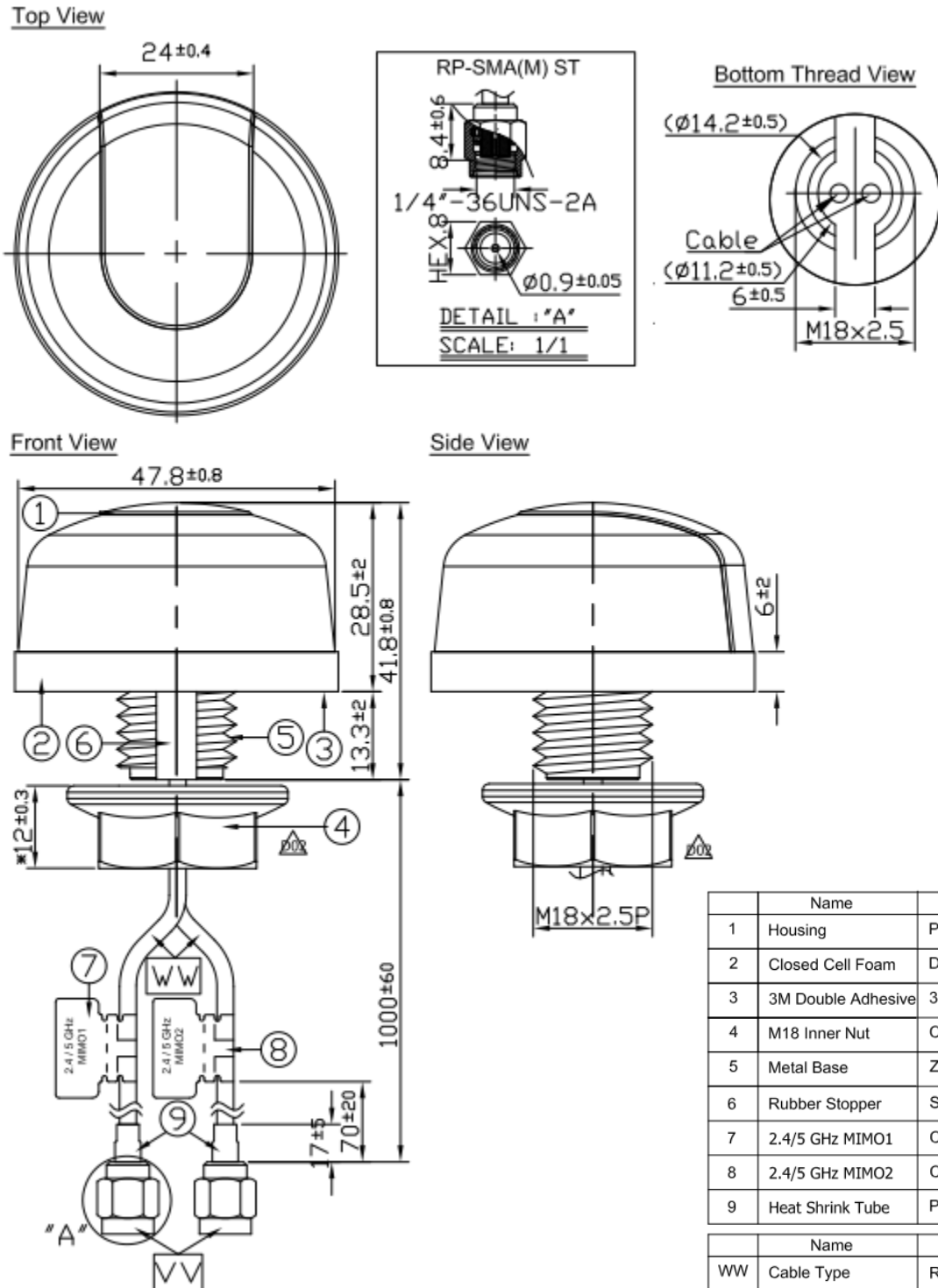
Figure 23. Antenna Drawing
