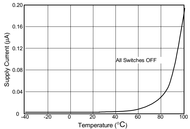
Fig. 6 OFF-State Current vs. Temperature
