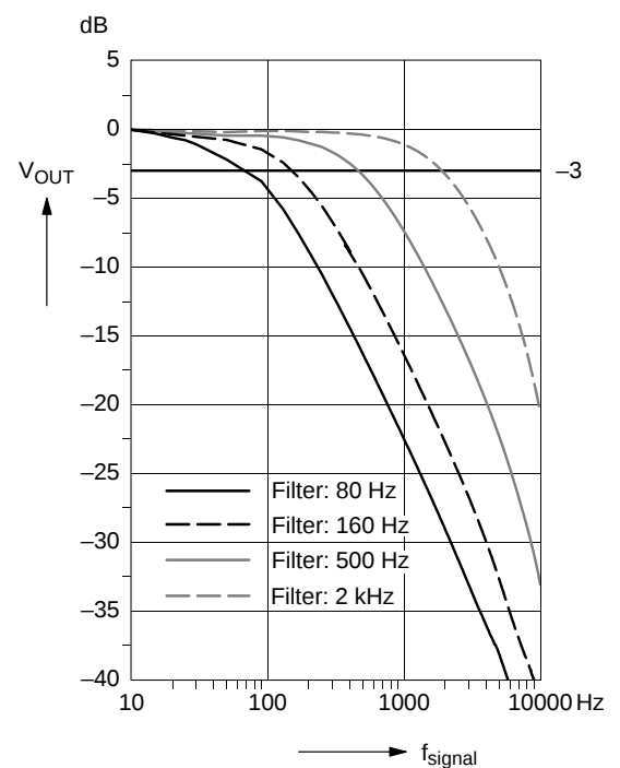
Fig. 3-5: Typical output voltage versus signal frequency
