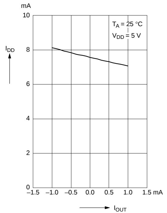
Fig. 3-4: Typical current consumption versus output current
