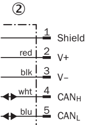
② Connector M12, 5-pin, A-coded
