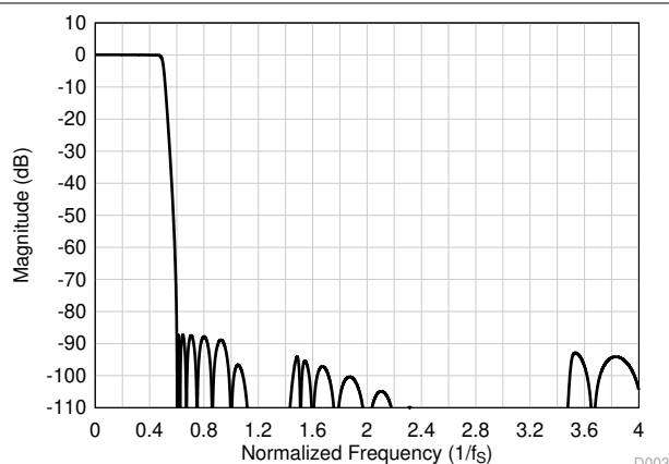
Figure 8-49. Ultra-Low-Latency Decimation Filter Magnitude Response
