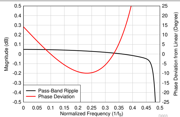
Figure 8-50. Ultra-Low-Latency Decimation Filter Pass-Band Ripple and Phase Deviation
