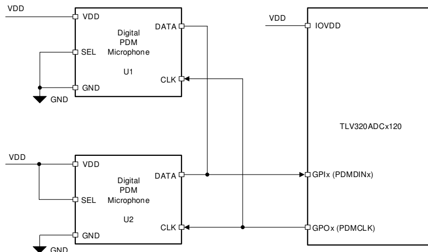
Figure 8-64. Digital PDM Microphones Connection Diagram to the TLV320ADC3120
