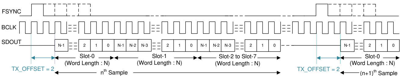
Figure 8-2. TDM Mode Protocol Timing (TX_OFFSET = 2)
