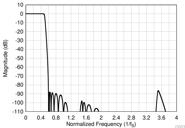
Figure 8-55. Ultra-Low-Latency Decimation Filter Magnitude Response
