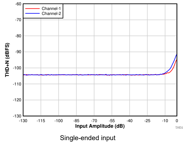
Figure 7-5. THD+N vs Input Amplitude
