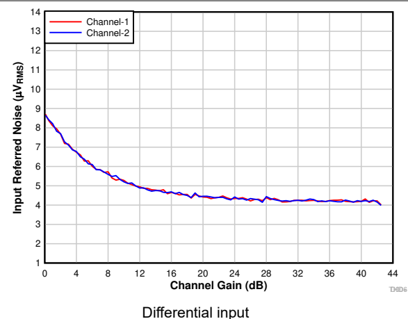
Figure 7-9. Input-Referred Noise vs Channel Gain
