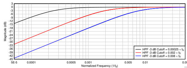
Figure 8-17. HPF Filter Frequency Response Plot
