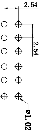
RECOMMENDED PCB LAYOUT COMPONENT SIDE VIEW
