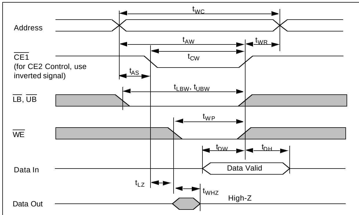
FIGURE 8: Timing Waveform of Write Cycle (2) (CE1 Control)
