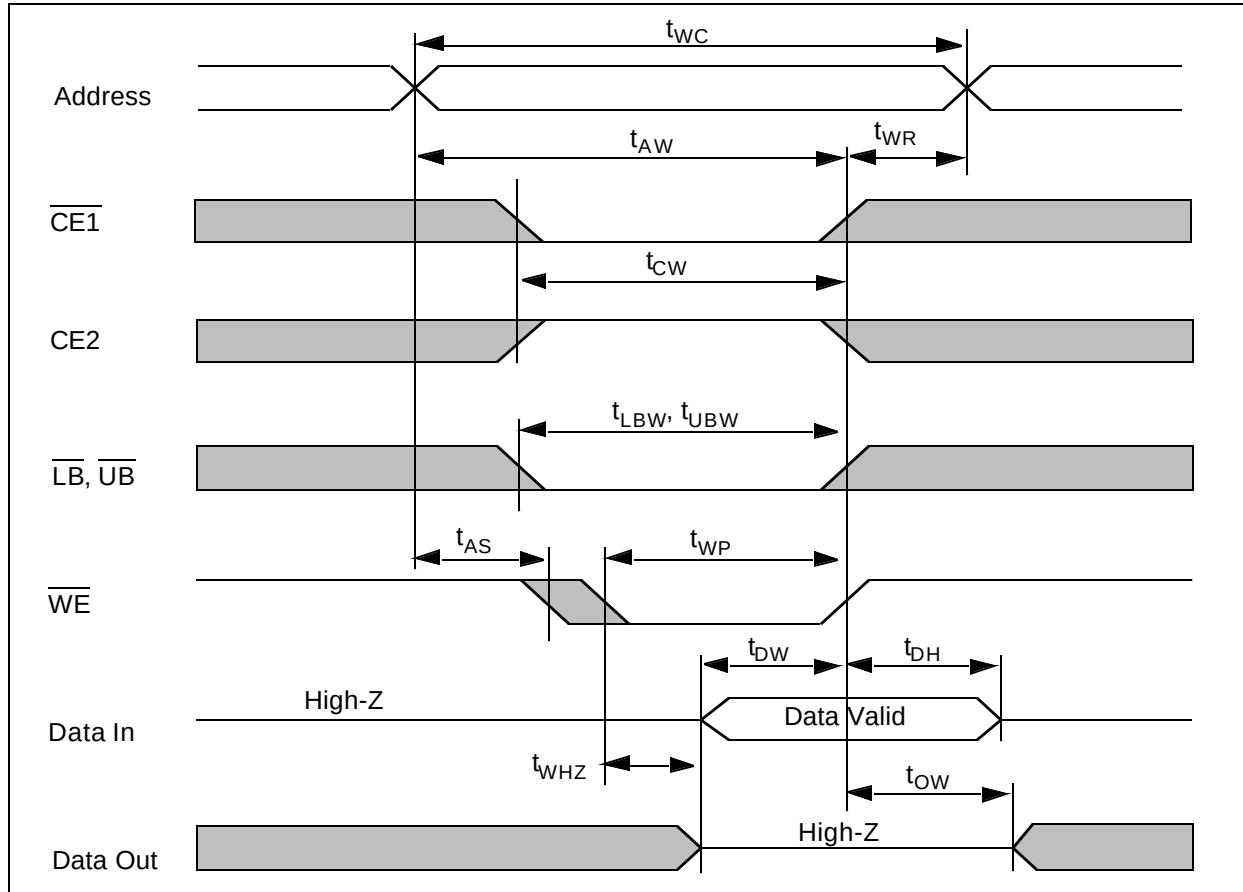
FIGURE 8: Timing Waveform of Write Cycle (2) (CE1 Control)
