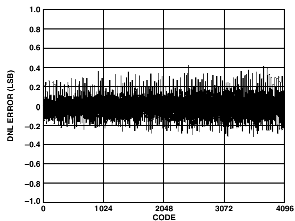
TPC 4. Typical DNL For the AD7453 for V_{DD} = 5 \text{ V}
