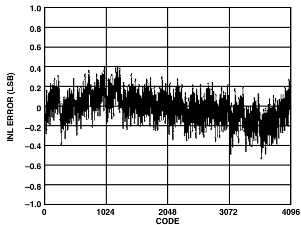
TPC 5. Typical INL For the AD7453 for V_{DD} = 5 \text{ V}
