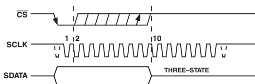
Figure 14. Entering Power-Down Mode
