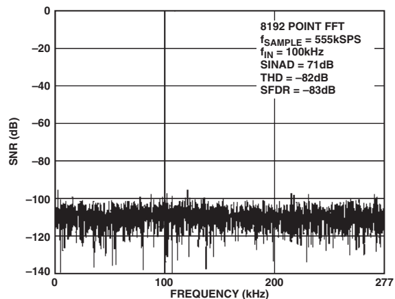
TPC 3. Dynamic Performance for V_{DD} = 5 \text{ V}
