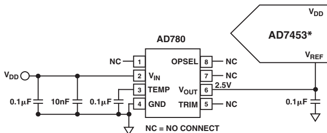
Figure 11. Typical V_{REF} Connection Diagram for V_{DD} = 5\text{ V}
