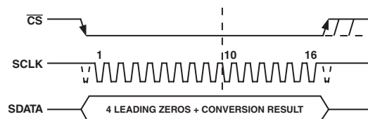
Figure 13. Normal Mode Operation
