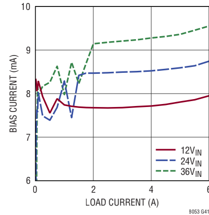
LTM8053 BIAS Current vs Load Current, V_{OUT} = 8\text{V} , BIAS = 5V
