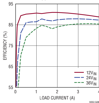
LTM8053 Efficiency vs Load Current, V_{OUT} = 5\text{V} , BIAS = 5V
