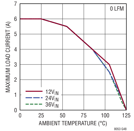
LTM8053 Derating, V_{OUT} = 0.97\text{V} , BIAS = 5V, DC1934A Demo Board
