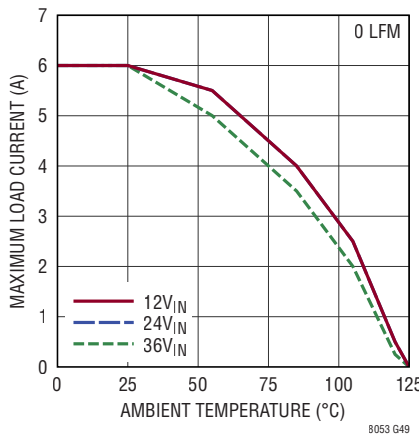
LTM8053 Derating, V_{OUT} = 1.2\text{V} , BIAS = 5V, DC1934A Demo Board
