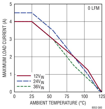
LTM8053 Derating, V_{OUT} = -5\text{V} , BIAS Tied to LTM8053 GND, DC1934A Demo Board
