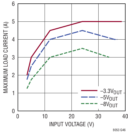
LTM8053 Maximum Load Current vs V_{IN} , BIAS Open
