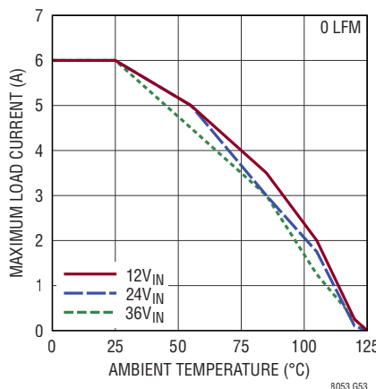
LTM8053 Derating, V_{OUT} = 2.5\text{V} , BIAS = 5V, DC1934A Demo Board
