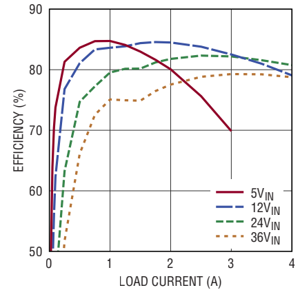
LTM8053 Efficiency vs Load Current, V_{OUT} = -3.3\text{V} , BIAS Tied to LTM8053 GND
