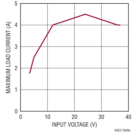
Maximum Load Current vs V IN . BIAS Open
