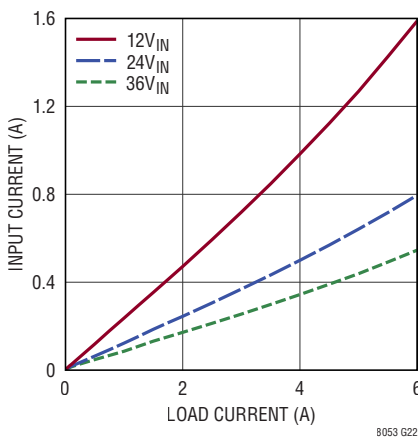
LTM8053 Input vs Load Current V_{OUT} = 2.5\text{V} , \text{BIAS} = 5\text{V}
