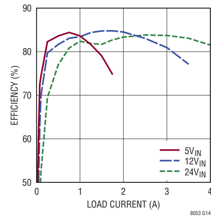
LTM8053 Efficiency vs Load Current, V_{OUT} = -8\text{V} , BIAS Tied to LTM8053 GND
