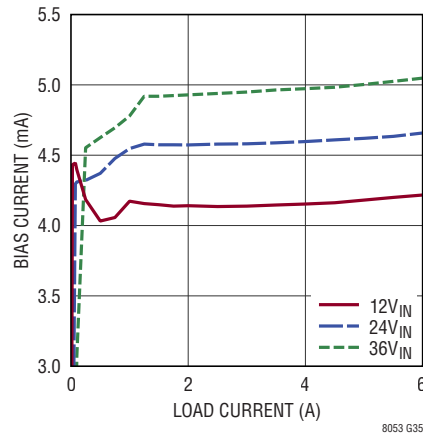
LTM8053 BIAS Current vs Load Current V_{OUT} = 1.5\text{V} , BIAS = 5V
