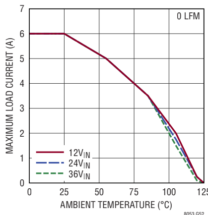
LTM8053 Derating, V_{OUT} = 2\text{V} , BIAS = 5V, DC1934A Demo Board
