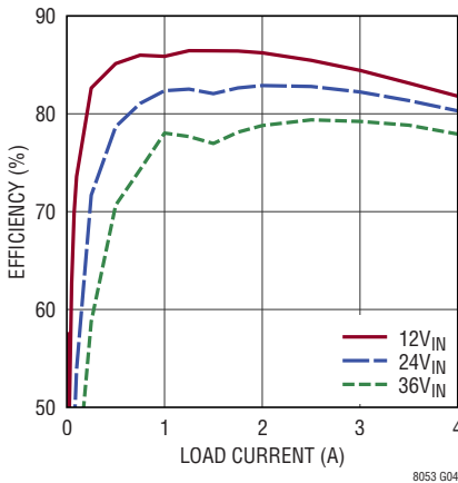
LTM8053 Efficiency vs Load Current, V_{OUT} = 1.8\text{V} , BIAS = 5V
