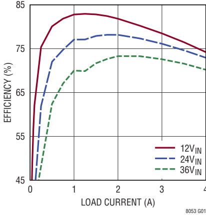
LTM8053 Efficiency vs Load Current, V_{OUT} = 0.97\text{V} , BIAS = 5V
