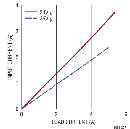
LTM8053 Input vs Load Current V_{OUT} = 15\text{V} , \text{BIAS} = 5\text{V}
