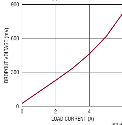
LTM8053 Dropout Voltage vs Load Current, V_{OUT} = 5\text{V} , BIAS = 5V
