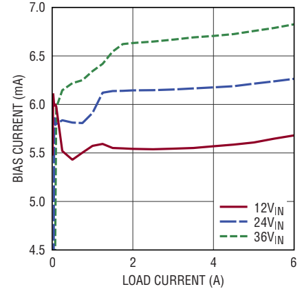
LTM8053 BIAS Current vs Load Current, V_{OUT} = 3.3\text{V} , BIAS = 5V
