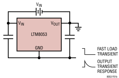
Figure 1b. Any Output Voltage Transient Appears on LTM8053/LTM8053-1 GND
