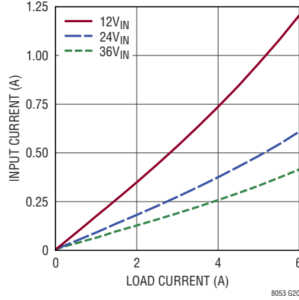
LTM8053 Input vs Load Current V_{OUT} = 1.8\text{V} , \text{BIAS} = 5\text{V}
