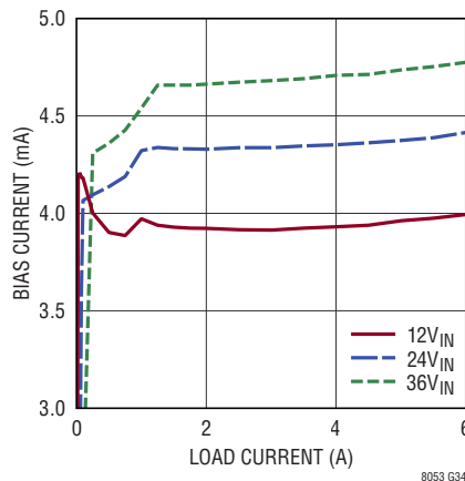
LTM8053 BIAS Current vs Load Current V_{OUT} = 1.2\text{V} , BIAS = 5V
