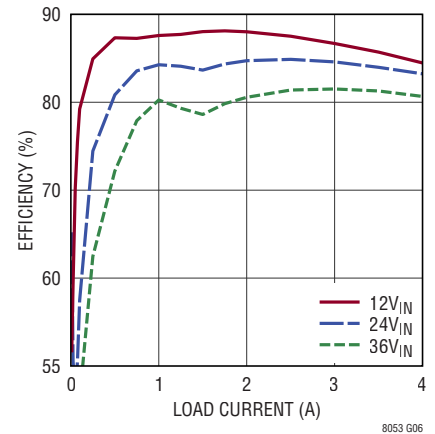
LTM8053 Efficiency vs Load Current, V_{OUT} = 2.5\text{V} , BIAS = 5V
