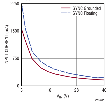
LTM8053 Input Current vs V_{IN} , V_{OUT} Short-Circuited
