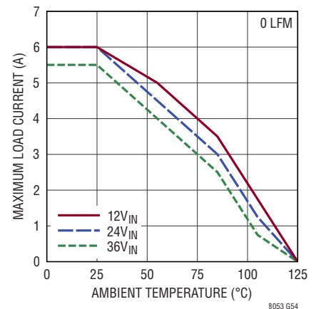
LTM8053 Derating, V_{OUT} = 3.3\text{V} , BIAS = 5V, DC1934A Demo Board
