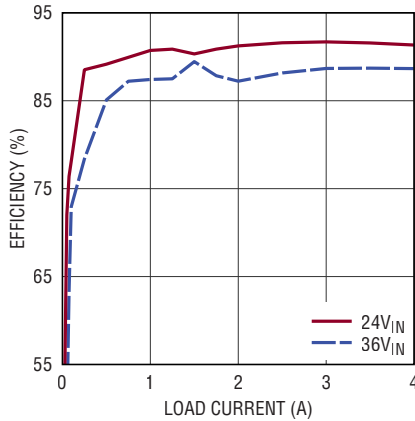
LTM8053 Efficiency vs Load Current, V_{OUT} = 12\text{V} , BIAS = 5V
