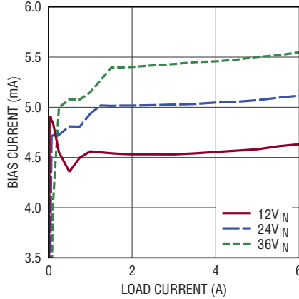
LTM8053 BIAS Current vs Load Current, V_{OUT} = 2\text{V} , BIAS = 5V
