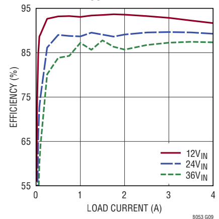
LTM8053 Efficiency vs Load Current, V_{OUT} = 8\text{V} , BIAS = 5V
