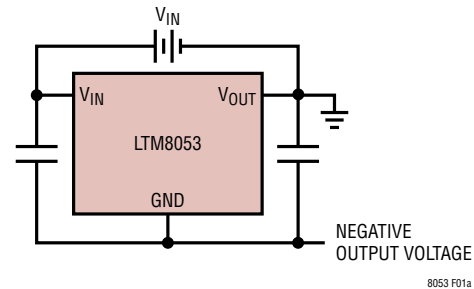
Figure 1a. The LTM8053/LTM8053-1 Can Be Used to Generate a Negative Voltage
