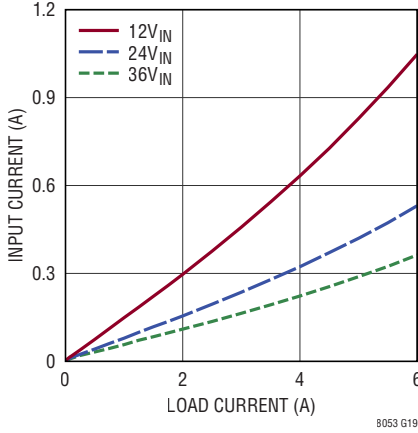
LTM8053 Input vs Load Current V_{OUT} = 1.5\text{V} , \text{BIAS} = 5\text{V}
