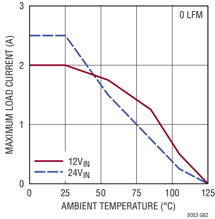
LTM8053 Derating, V_{OUT} = -12\text{V} , BIAS Tied to LTM8053 GND, DC1934A Demo Board
