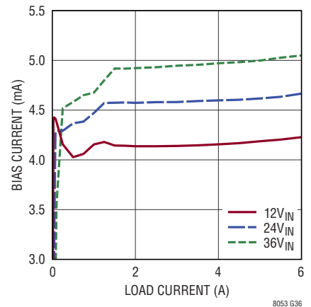
LTM8053 BIAS Current vs Load Current V_{OUT} = 1.8\text{V} , BIAS = 5V
