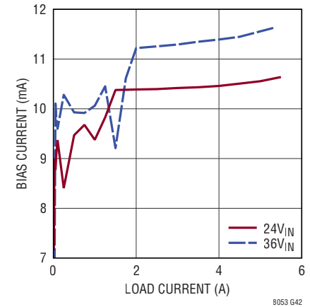
LTM8053 BIAS Current vs Load Current, V_{OUT} = 12\text{V} , BIAS = 5V
