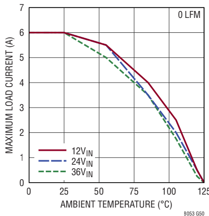
LTM8053 Derating, V_{OUT} = 1.5\text{V} , BIAS = 5V, DC1934A Demo Board
