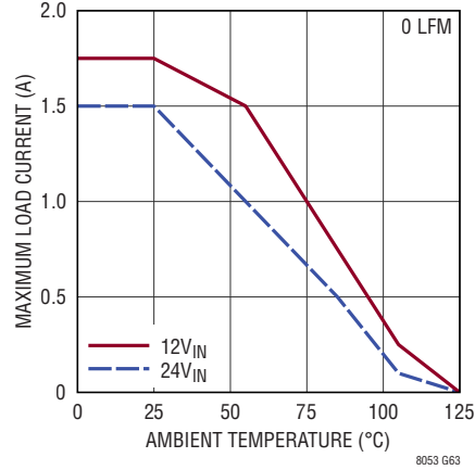
LTM8053 Derating, V_{OUT} = -15\text{V} , BIAS Tied to LTM8053 GND, DC1934A Demo Board
