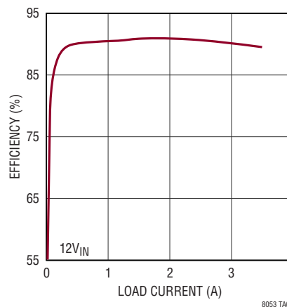
Efficiency, V OUT = 5V
