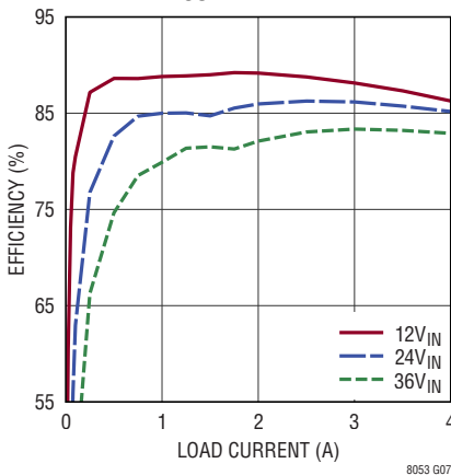
LTM8053 Efficiency vs Load Current, V_{OUT} = 3.3\text{V} , BIAS = 5V
