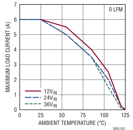
LTM8053 Derating, V_{OUT} = 1.8\text{V} , BIAS = 5V, DC1934A Demo Board
