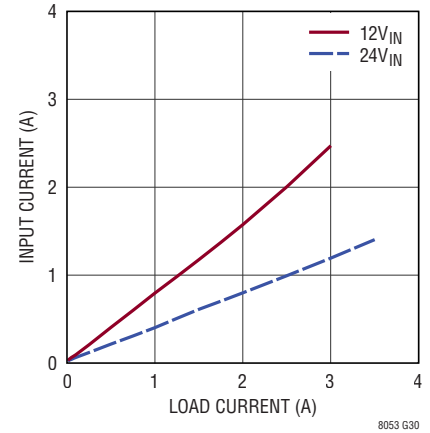
LTM8053 Input vs Load Current V_{OUT} = -8\text{V} , BIAS Tied to LTM8053 GND
