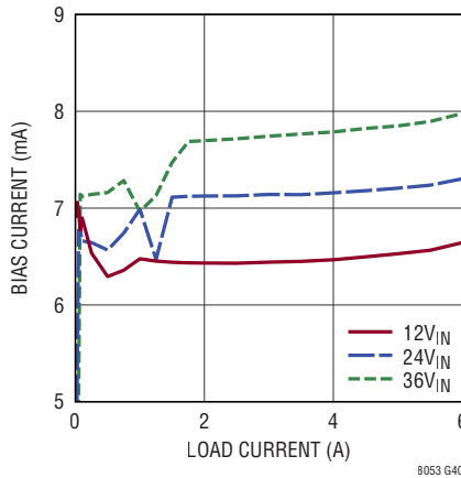
LTM8053 BIAS Current vs Load Current, V_{OUT} = 5\text{V} , BIAS = 5V
