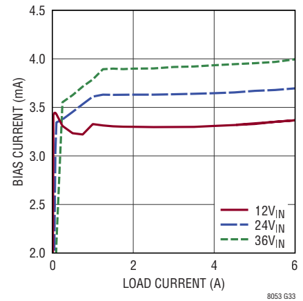
LTM8053 BIAS Current vs Load Current V_{OUT} = 0.97\text{V} , BIAS = 5V
