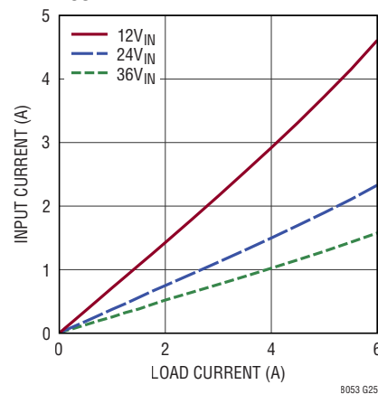
LTM8053 Input vs Load Current V_{OUT} = 8\text{V} , \text{BIAS} = 5\text{V}
