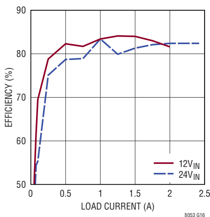
LTM8053 Efficiency vs Load Current, V_{OUT} = -15\text{V} , BIAS Tied to LTM8053 GND
