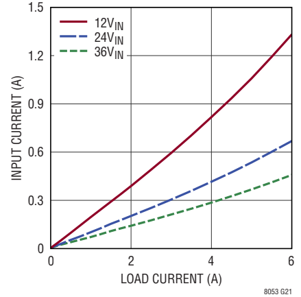
LTM8053 Input vs Load Current V_{OUT} = 2\text{V} , \text{BIAS} = 5\text{V}
