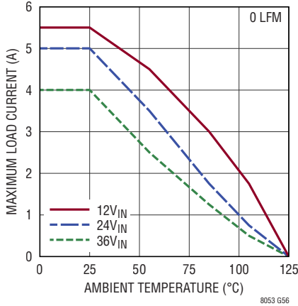
LTM8053 Derating, V_{OUT} = 8\text{V} , BIAS = 5V, DC1934A Demo Board
