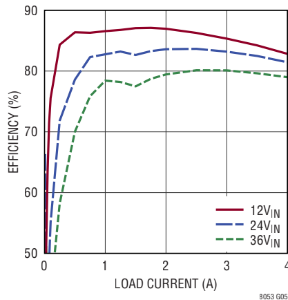
LTM8053 Efficiency vs Load Current, V_{OUT} = 2\text{V} , BIAS = 5V
