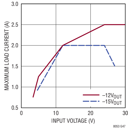
LTM8053 Maximum Load Current vs V_{IN} , BIAS Open
