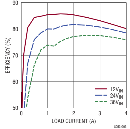
LTM8053 Efficiency vs Load Current, V_{OUT} = 1.5\text{V} , BIAS = 5V
