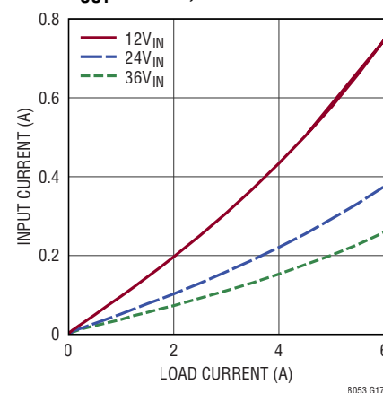
LTM8053 Input vs Load Current V_{OUT} = 0.97\text{V} , BIAS = 5V
