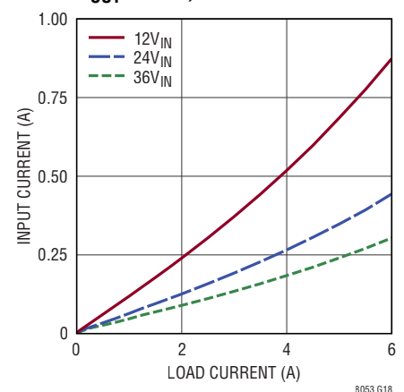
LTM8053 Input vs Load Current V_{OUT} = 1.2\text{V} , BIAS = 5V
