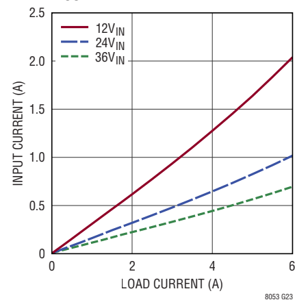
LTM8053 Input vs Load Current V_{OUT} = 3.3\text{V} , \text{BIAS} = 5\text{V}
