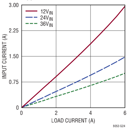
LTM8053 Input vs Load Current V_{OUT} = 5\text{V} , \text{BIAS} = 5\text{V}
