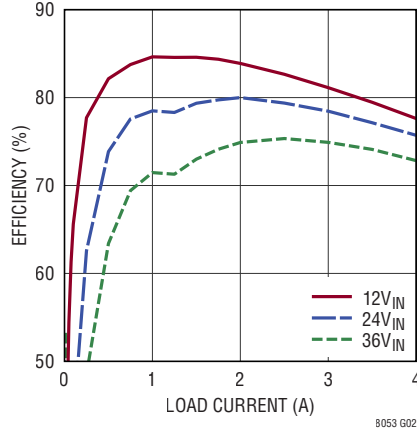
LTM8053 Efficiency vs Load Current, V_{OUT} = 1.2\text{V} , BIAS = 5V
