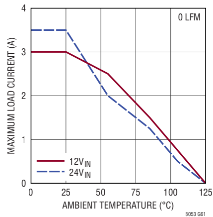
LTM8053 Derating, V_{OUT} = -8\text{V} , BIAS Tied to LTM8053 GND, DC1934A Demo Board
