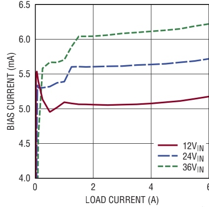
LTM8053 BIAS Current vs Load Current, V_{OUT} = 2.5\text{V} , BIAS = 5V
