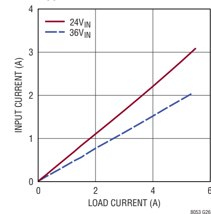
LTM8053 Input vs Load Current V_{OUT} = 12\text{V} , \text{BIAS} = 5\text{V}
