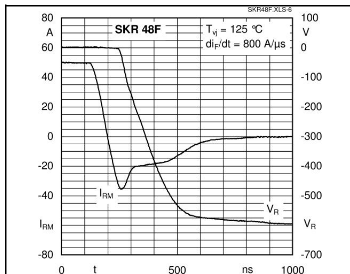
Fig. 6 Typ. reverse recovery characteristics
