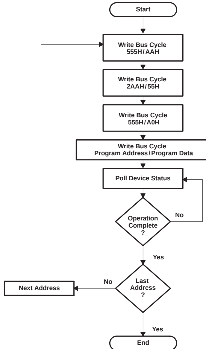
Figure 1. Program Algorithm
