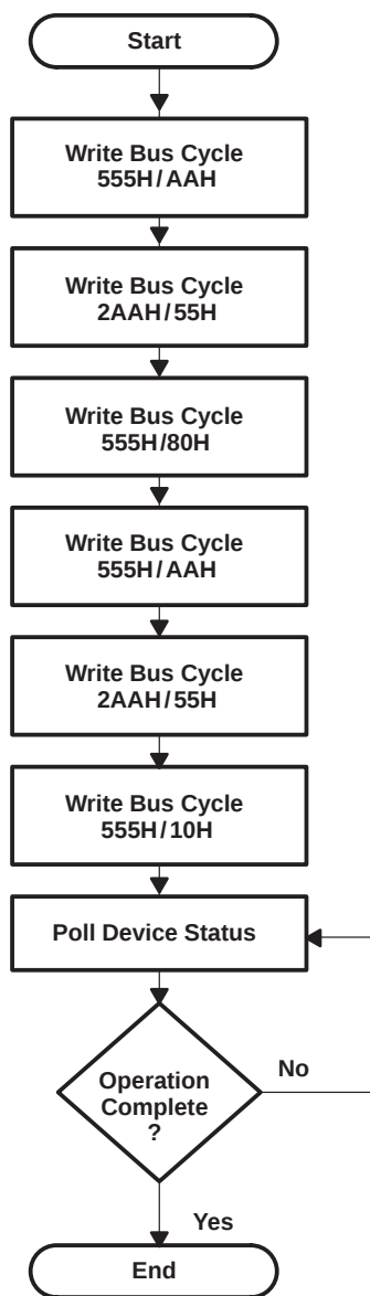
Figure 2. Chip-Erase Algorithm
