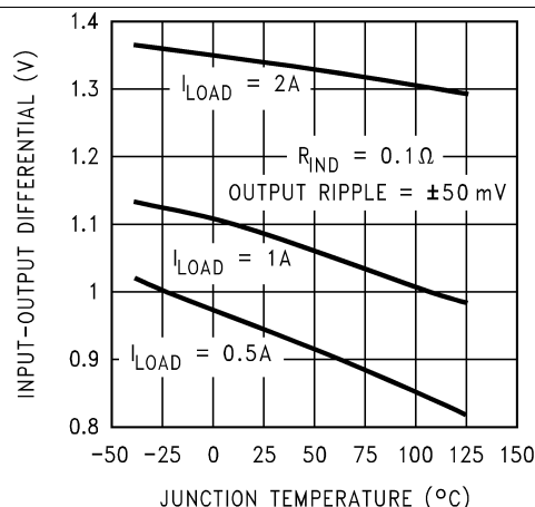
Figure 6. Dropout Voltage
