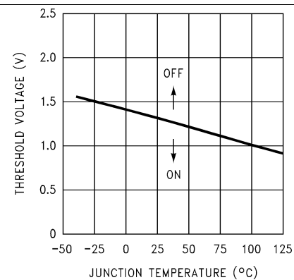
Figure 12. \overline{\text{ON}} /OFF Threshold Voltage
