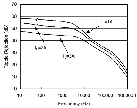
Ripple Rejection
