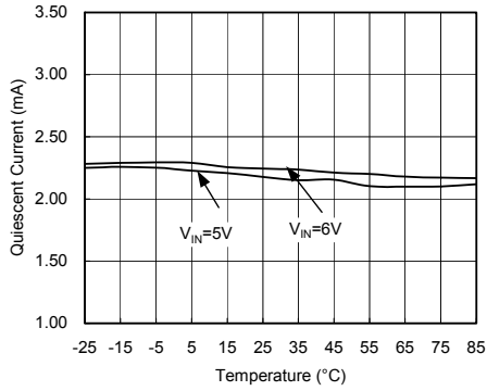
G1085-25 Quiescent Current vs. Temperature
