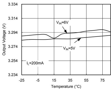
G1085-33-Output Voltage vs. Temperature
