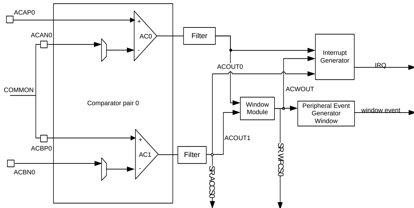
Figure 27-2. Analog Comparator Interface in Window Mode
