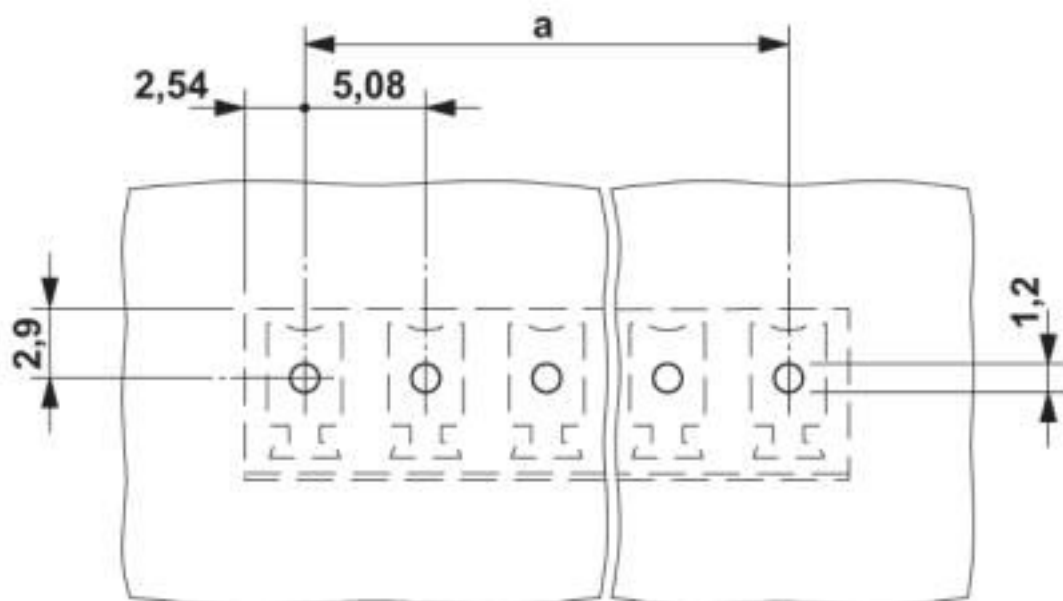
Drilling diagram
