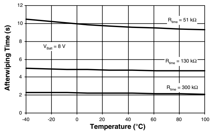
Figure 8-2. After-wiping Time = f(T) ; C_t = 22 \mu F ; V_{Batt} = 8V
