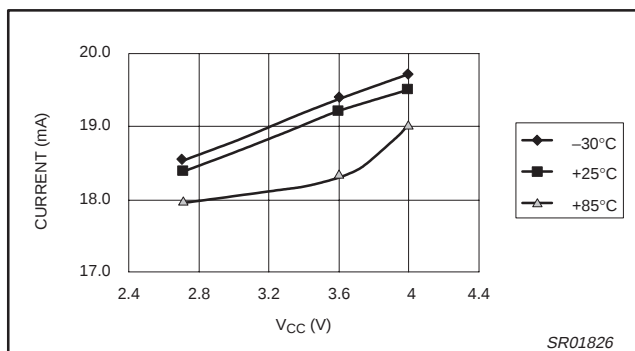
Figure 4. PCS Idle (with doubled LO out) current
