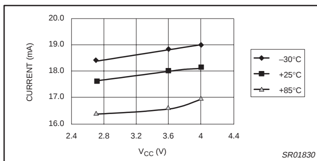
Figure 8. Cellular CDMA Rx Idle current
