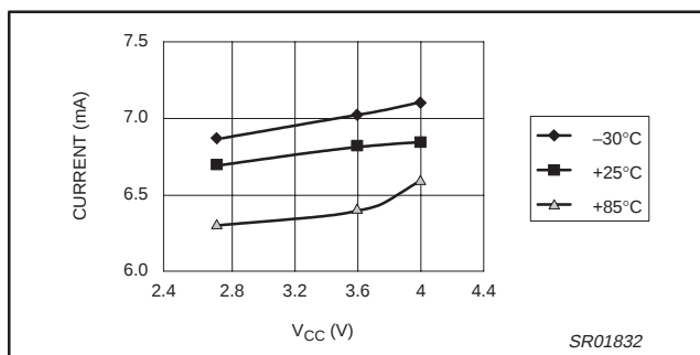
Figure 10. Cellular FM Rx Idle current
