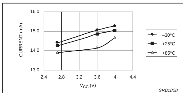
Figure 6. PCS Rx Idle current
