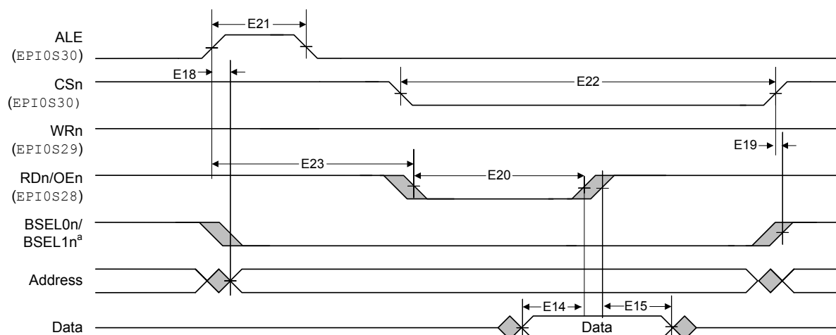
Figure 29-21. Host-Bus 8/16 Asynchronous Mode Read Timing
