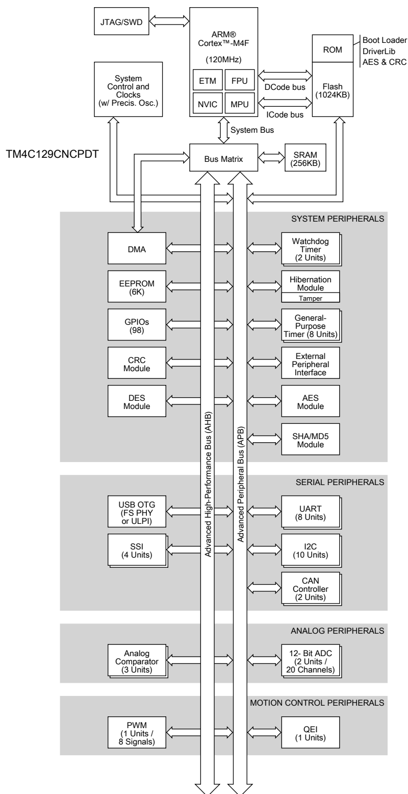
Figure 1-1. Tiva™ TM4C129CNPDT Microcontroller High-Level Block Diagram
