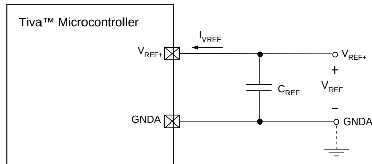
Figure 29-28. ADC External Reference Filtering
