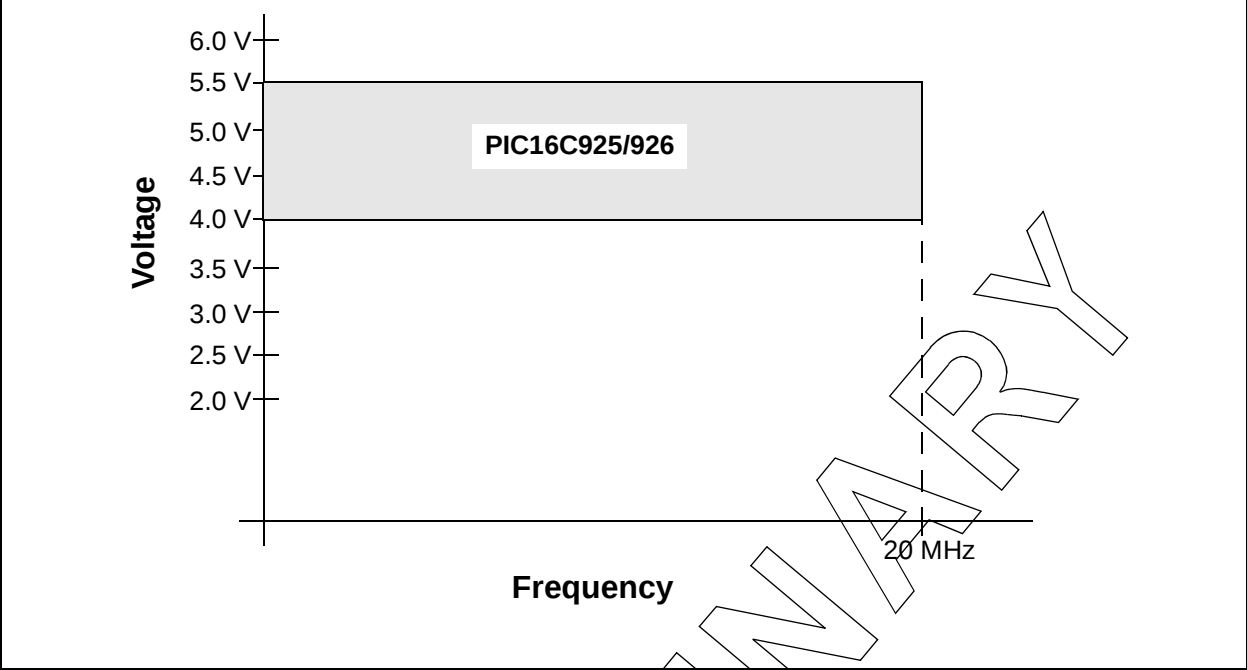
FIGURE 15-1: PIC16C925/926 VOLTAGE-FREQUENCY GRAPH
