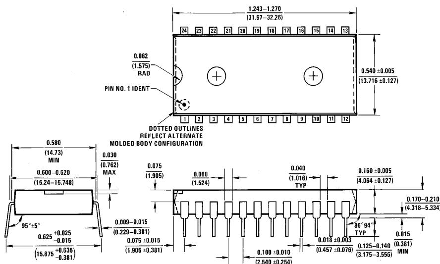
Order Number ADC10838CIN NS Package Number N24A
